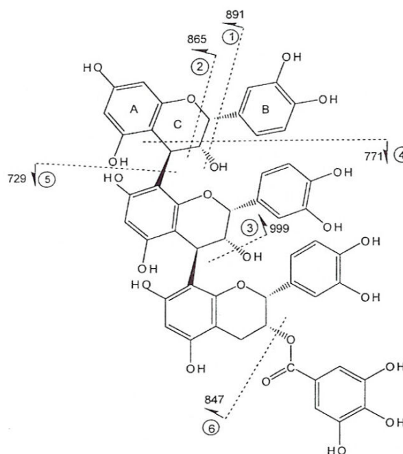
Trimer gallate, a trimer unit with one gallate substituent.
